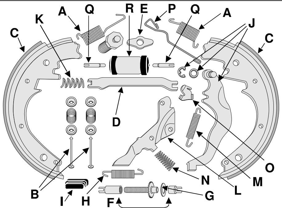
This drawing is a composite; it is intended to represent all models, both front and rear.
